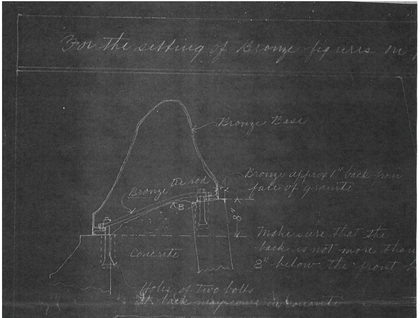
Detail from Allward's technical drawings illustrating how to set the bronze figures in place. 1928.
